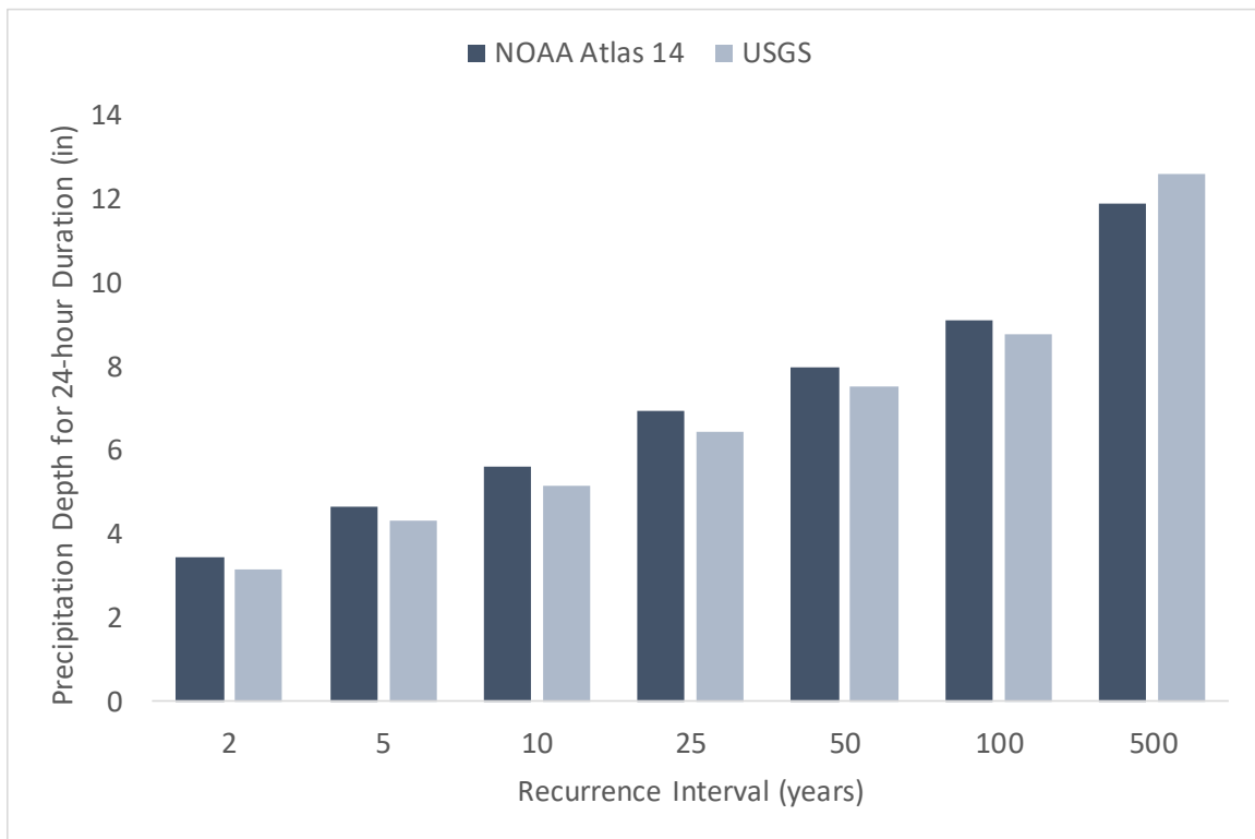
Figure 12. Comparison of NOAA Atlas 14 and USGS estimated precipitation depth for 24-hour duration storms for Parker County (inches)
