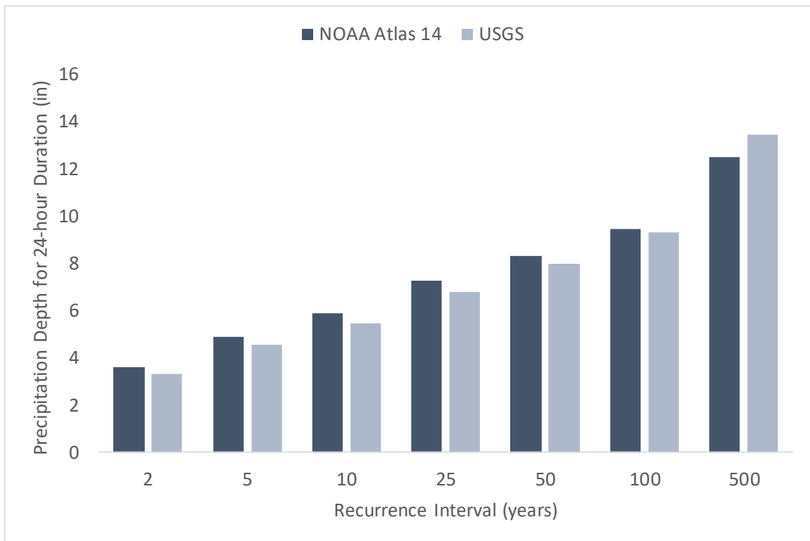
Figure 8. Comparison of NOAA Atlas 14 and USGS estimated precipitation depth for 24-hour duration storms for Johnson County (inches)
