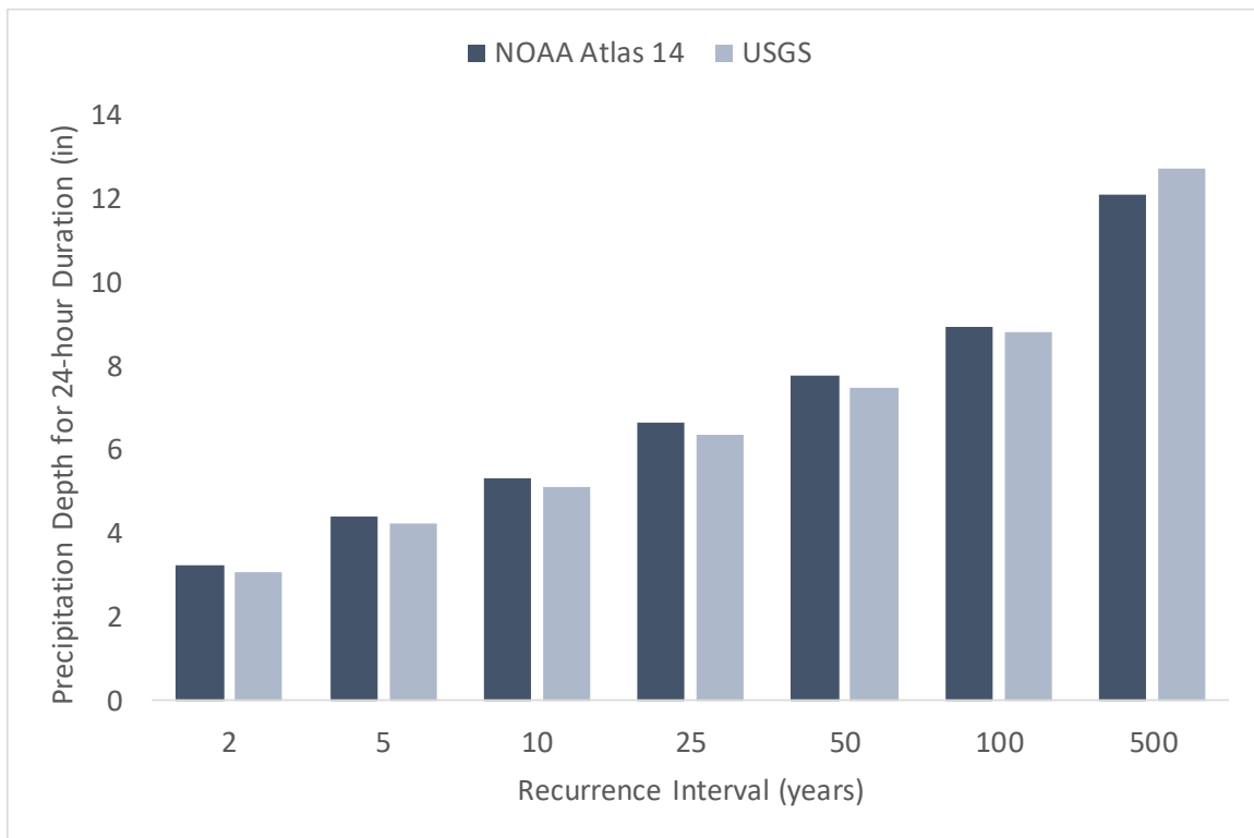
Figure 11. Comparison of NOAA Atlas 14 and USGS estimated precipitation depth for 24-hour duration storms for Palo Pinto County (inches)
