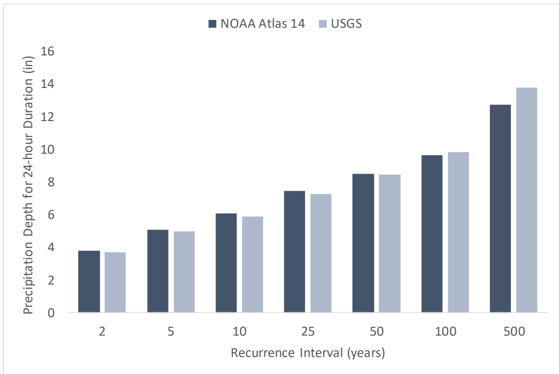
Figure 13. Comparison of NOAA Atlas 14 and USGS estimated precipitation depth for 24-hour duration storms for Rockwall County (inches)
