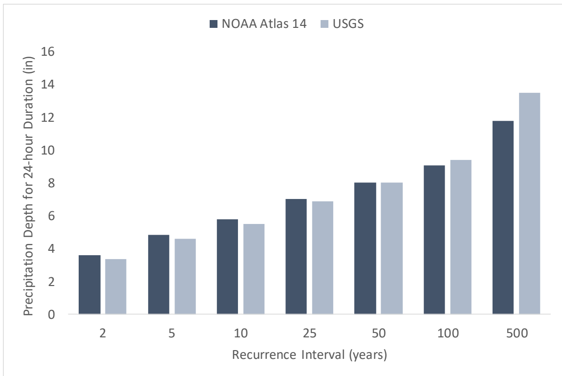
Figure 3. Comparison of NOAA Atlas 14 and USGS estimated precipitation depth for 24-hour duration storms for Denton County (inches)
