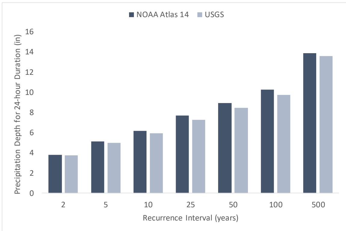
Figure 9. Comparison of NOAA Atlas 14 and USGS estimated precipitation depth for 24-hour duration storms for Kaufman County (inches)
