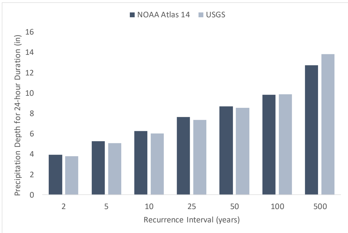
Figure 7. Comparison of NOAA Atlas 14 and USGS estimated precipitation depth for 24-hour duration storms for Hunt County (inches)
