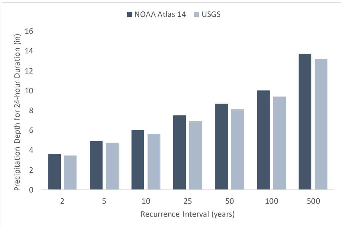
Figure 4. Comparison of NOAA Atlas 14 and USGS estimated precipitation depth for 24-hour duration storms for Ellis County (inches)
