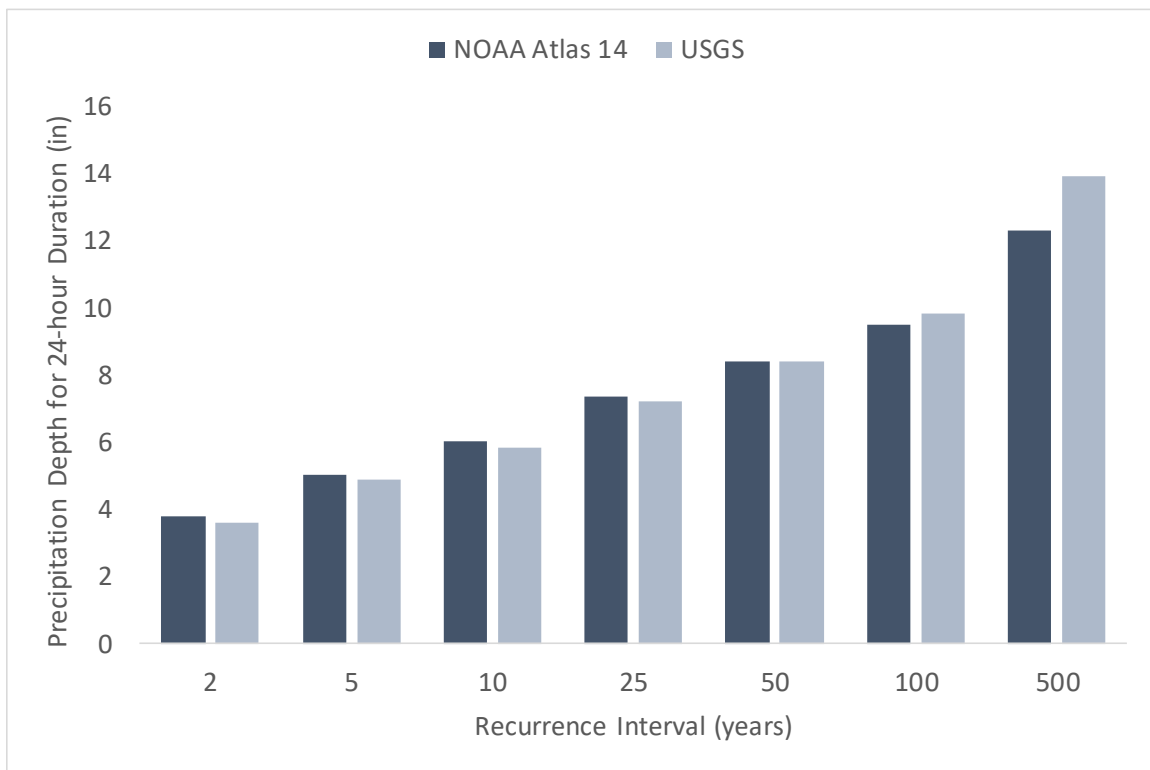
Figure 1. Comparison of NOAA Atlas 14 and USGS estimated precipitation depth for 24-hour duration storms for Collin County (inches)
