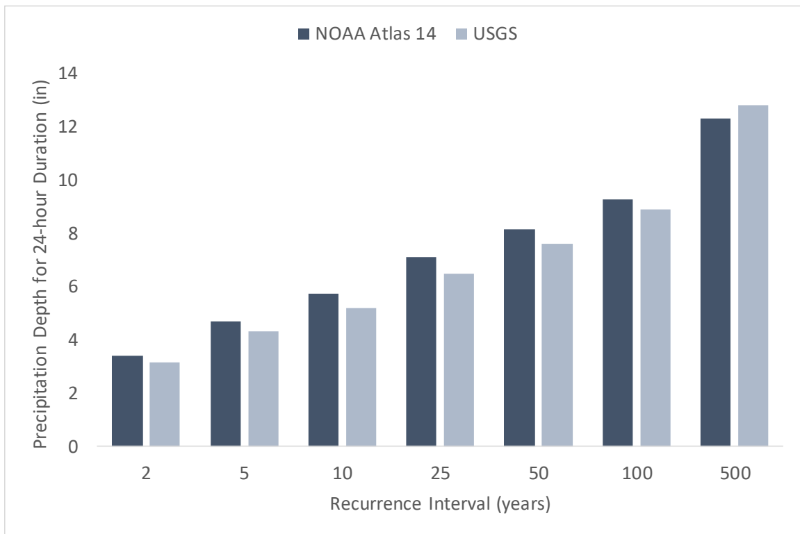
Figure 14. Comparison of NOAA Atlas 14 and USGS estimated precipitation depth for 24-hour duration storms for Somervell County (inches)
