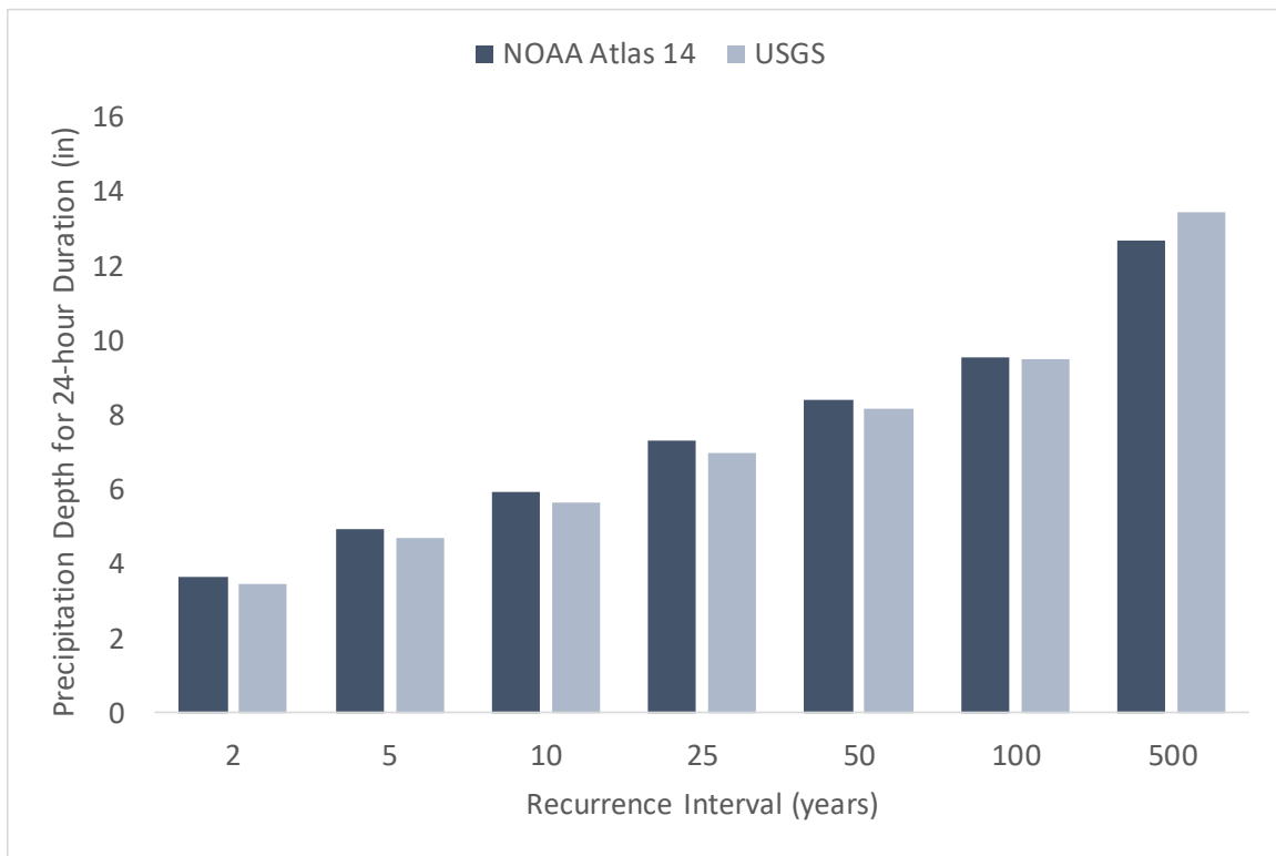
Figure 2. Comparison of NOAA Atlas 14 and USGS estimated precipitation depth for 24-hour duration storms for Dallas County (inches)
