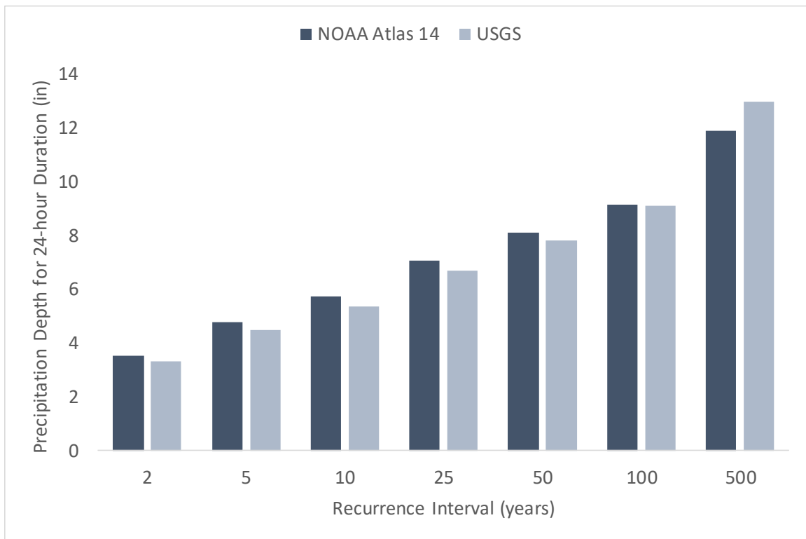
Figure 15. Comparison of NOAA Atlas 14 and USGS estimated precipitation depth for 24-hour duration storms for Tarrant County (inches)
