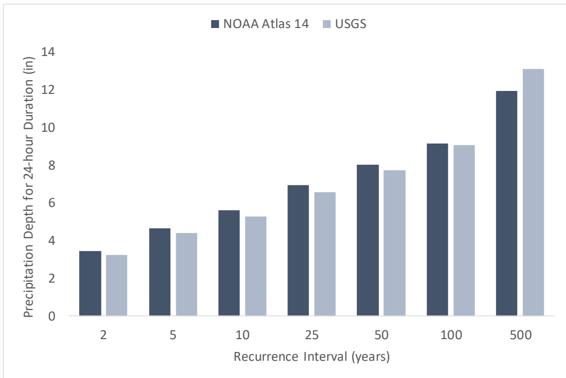
Figure 16. Comparison of NOAA Atlas 14 and USGS estimated precipitation depth for 24-hour duration storms for Wise County (inches)
