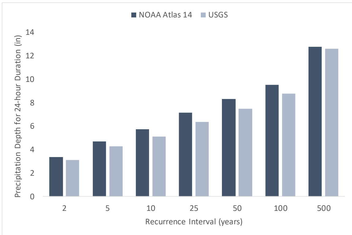
Figure 5. Comparison of NOAA Atlas 14 and USGS estimated precipitation depth for 24-hour duration storms for Erath County (inches)
