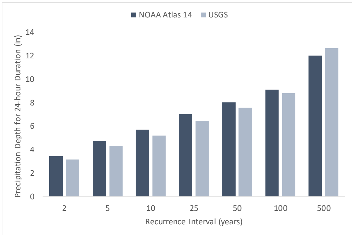
Figure 6. Comparison of NOAA Atlas 14 and USGS estimated precipitation depth for 24-hour duration storms for Hood County (inches)
