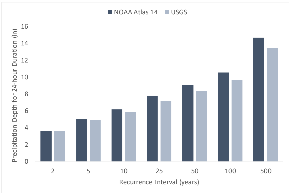
Figure 10. Comparison of NOAA Atlas 14 and USGS estimated precipitation depth for 24-hour duration storms for Navarro County (inches)
