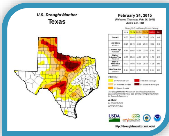
Figure 2. U.S. Drought Monitor for Texas February 24, 2015. Credit: NDMC
