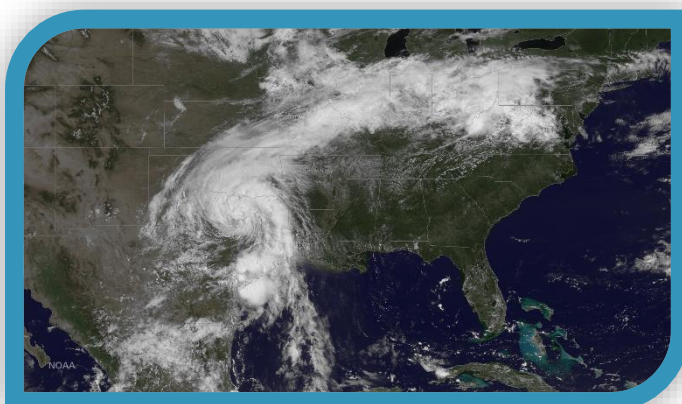
Figure 8. Satellite image (left) and total rainfall (right) from Tropical Storm Bill. Credit: IB Times (left) and iWeatherNet (right).
